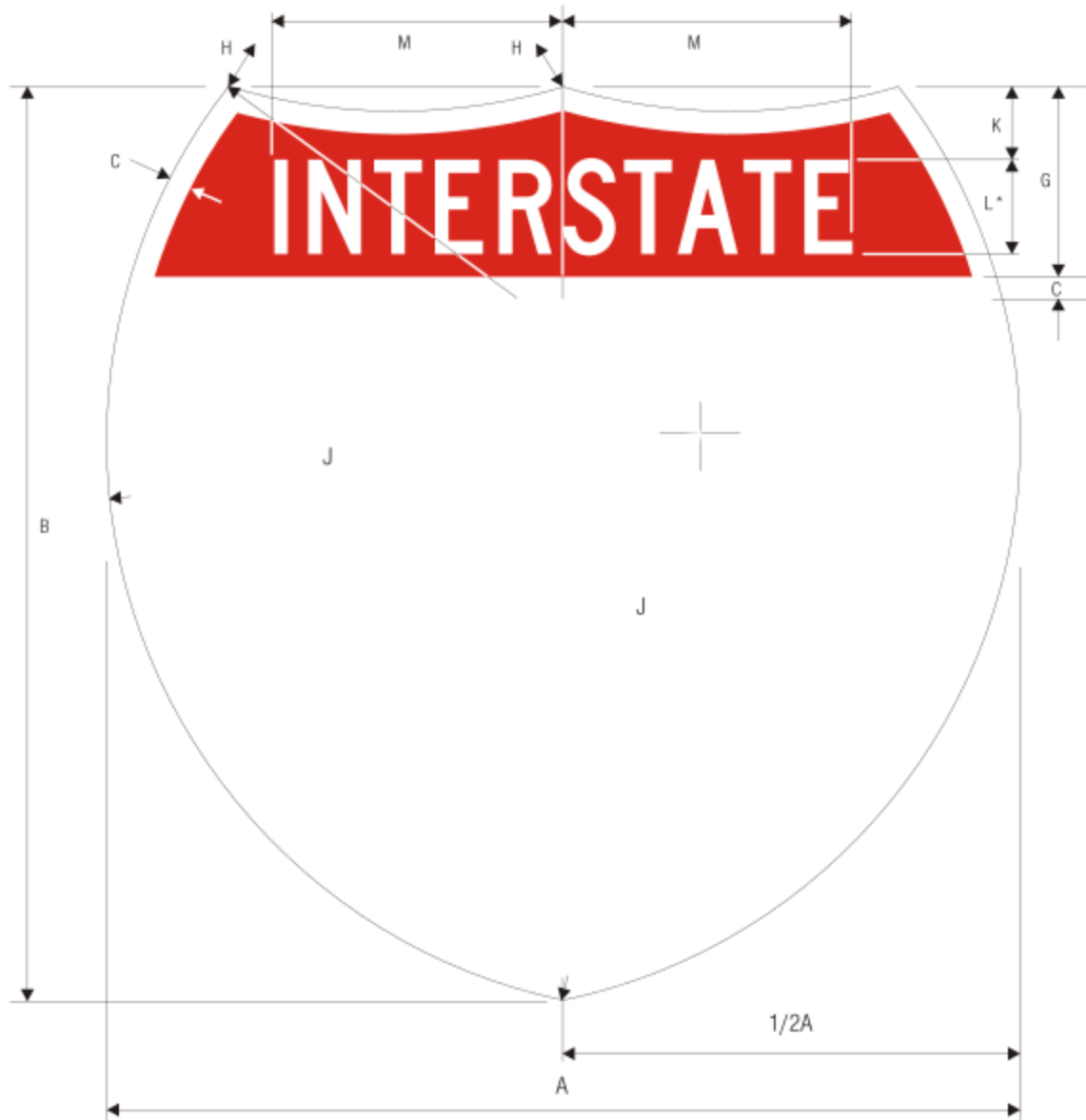
M1-1 INTERSTATE ROUTE RCOC MODIFIED
