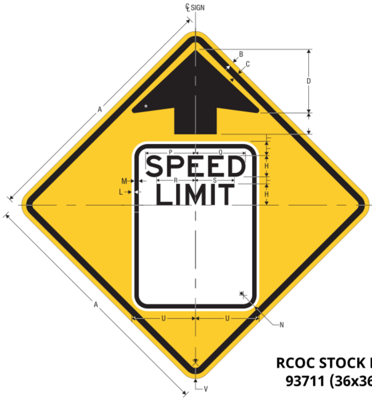
W3-5 REDUCED SPEED LIMIT AHEAD RCOC MODIFIED
