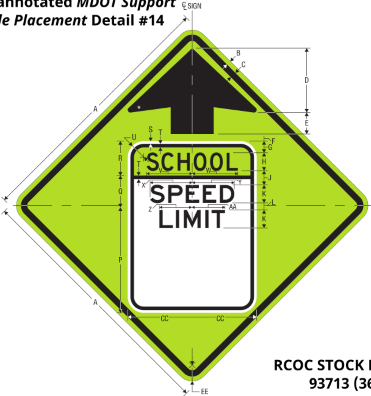
S4-5 REDUCED SCHOOL SPEED LIMIT AHEAD RCOC MODIFIED
